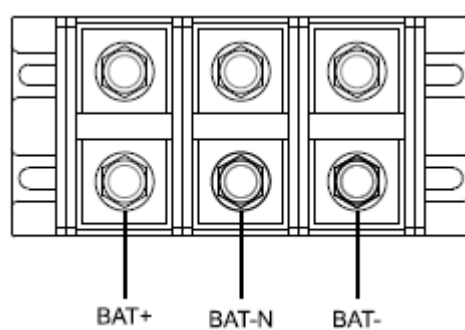
HV 60KL/80KL and LV 30KL/40KL 端子排示意图
